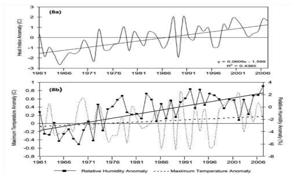
Figure 1: a) Heat Index Anomalies in Pakistan b) Maximum Temperature and Relative Humidity Anomalies for the Period 1961-2007
